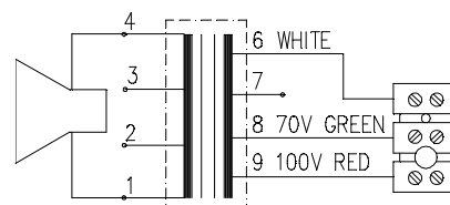
CIRCUIT DIAGRAM
