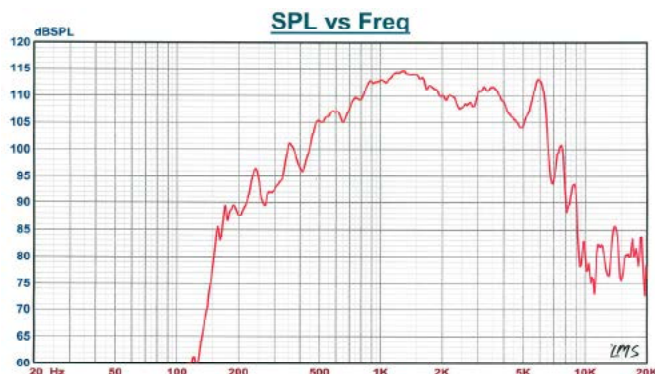
Sound pressure levels at 1W/1m in Tunnel-500
